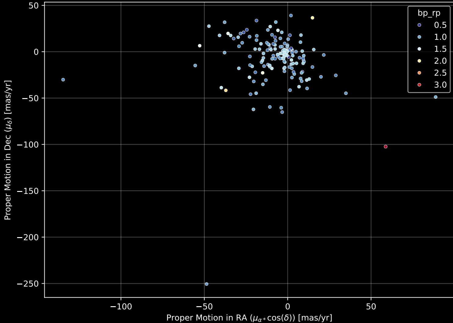
APOGEE DR17 Field: [045+40_MGA] Proper Motion Diagram (n= 152)
