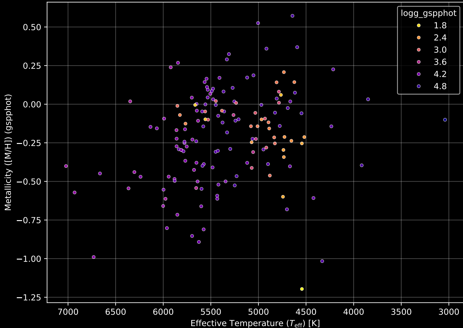
APOGEE DR17 Field: [045+40_MGA] Stellar Population Parameters (n= 152)
