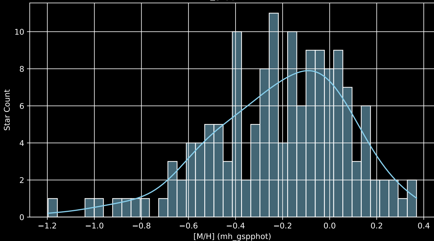
APOGEE DR17 Field: [045+40_MGA [M/H] (mh_gspphot) (n= 150)
