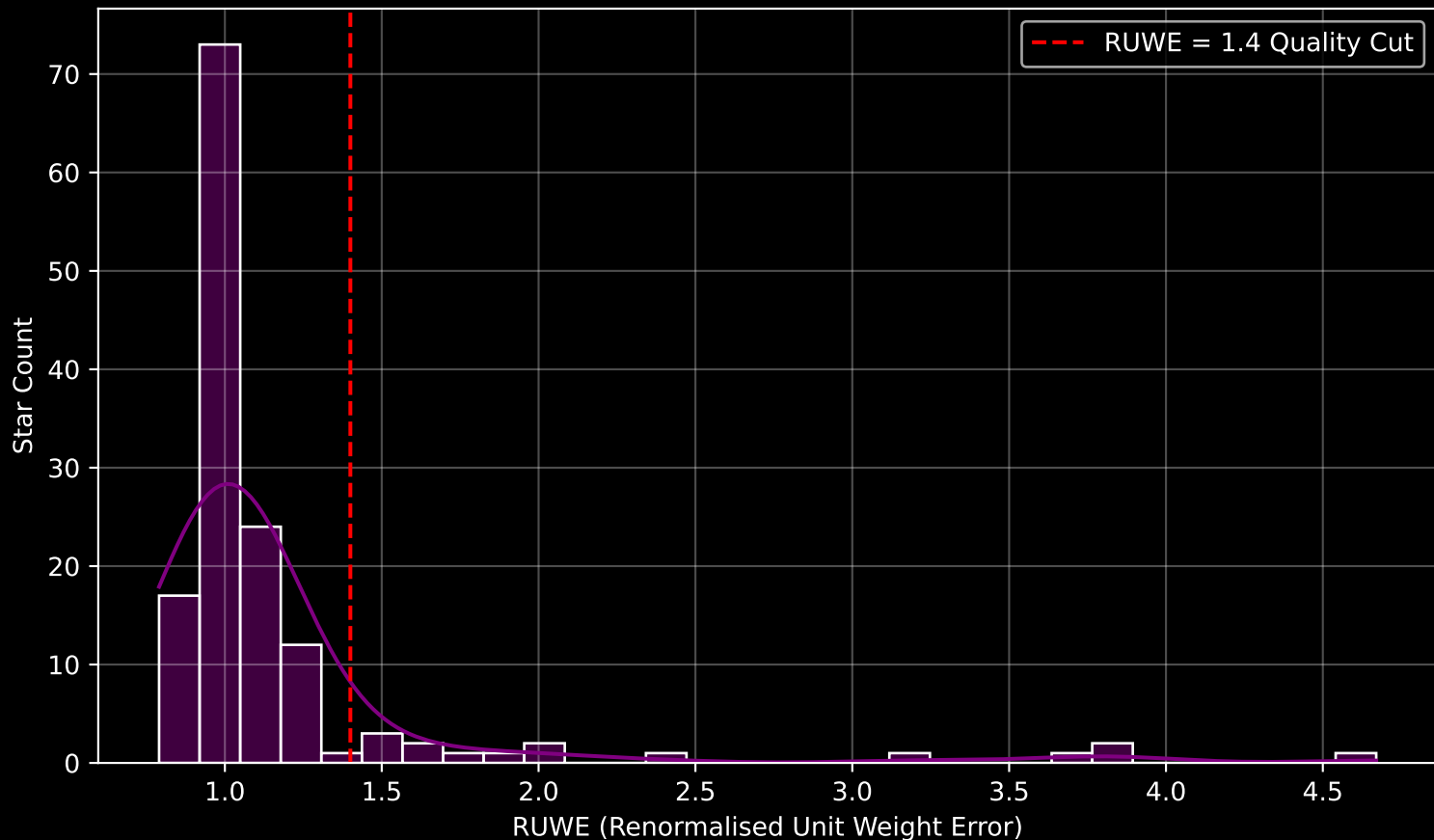
GAPOGEE DR17 Field [045+40_MGA] RUWE Distribution (n= 142)
