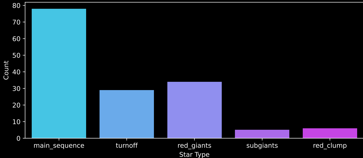
APOGEE DR17 Field: [045+40_MGA] Count plot of Star Type
