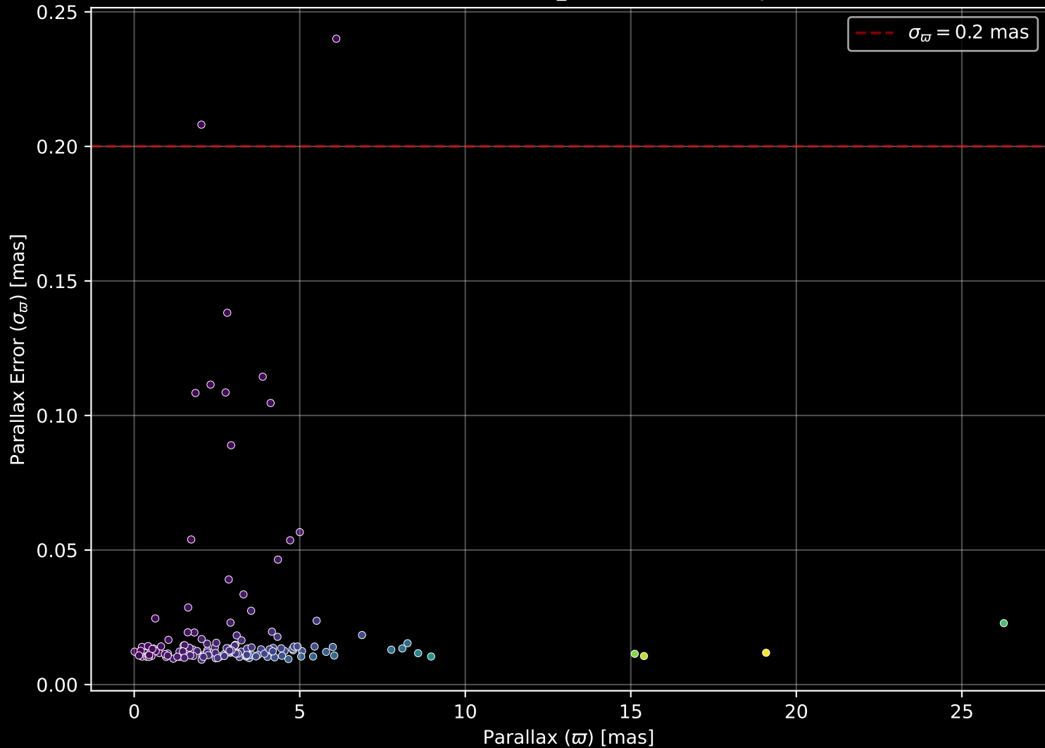
APOGEE DR17 Field: [045+40_MGA] Parallax Quality (n= 152)
